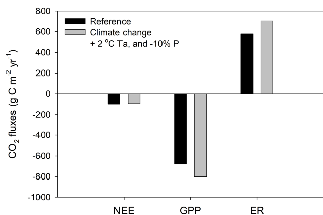
Figure 7. Simulated CO 2 fluxes under a scenario in which air temperature is increased year-round by 2 °C and precipitation is decreased by 10 %. Equilibrium model runs used the BDB 2013–2016 setup and Rivière-du-Loup 1994–2021 climate data.
